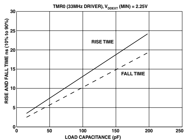
Figure 50. Typical Rise and Fall Times (10% to 90%) versus Load Capacitance for Driver C at V_{DDEXT} = 2.25\text{V}
