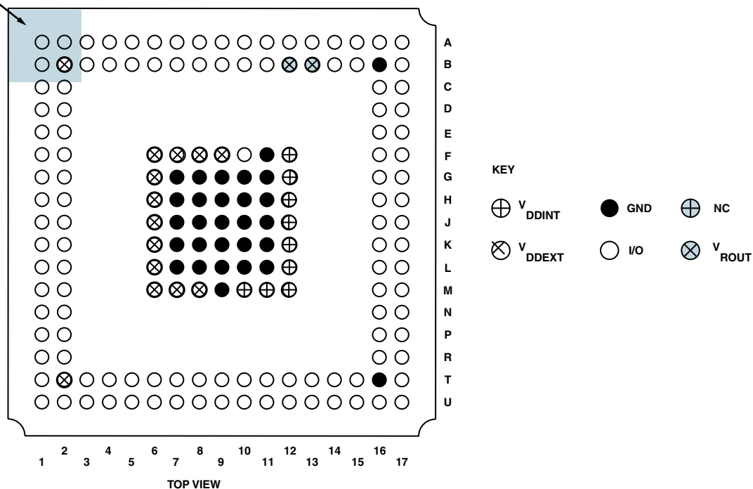
Figure 57. 169-Ball PBGA Ground Configuration (Top View)
