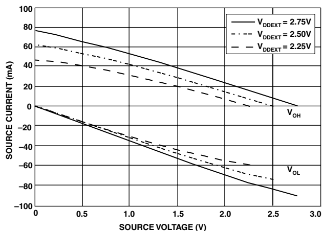
Figure 37. Drive Current D ( V_{DDEXT} = 2.5\text{ V} )
