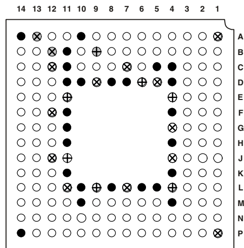
Figure 55. 160-Ball Mini-BGA Ground Configuration (Top View)
