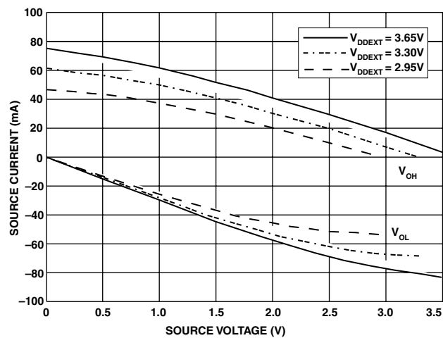
Figure 36. Drive Current C ( V_{DDEXT} = 3.3\text{ V} )
