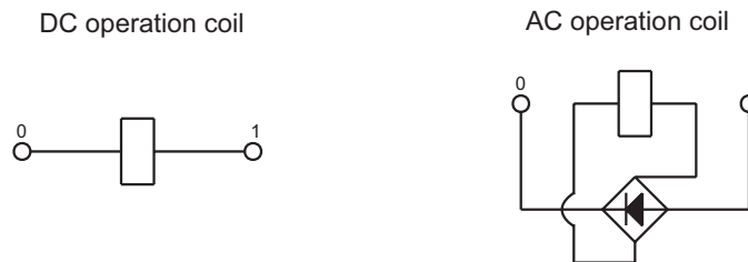
Coil Inner Circuit
