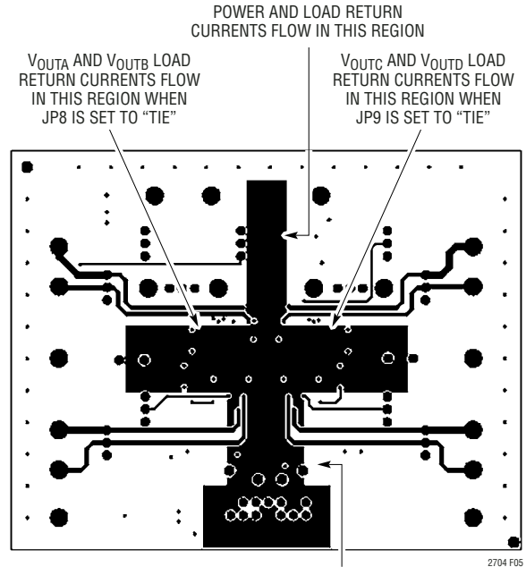
Figure 5. DC752A Load Return, Power Return and Digital Return
