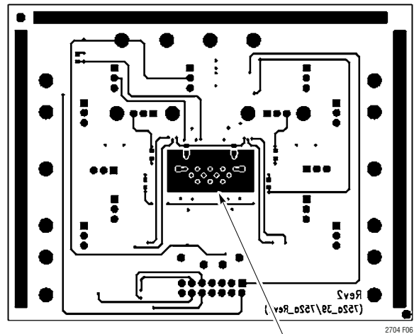
Figure 5. DC752A Load Return, Power Return and Digital Return
