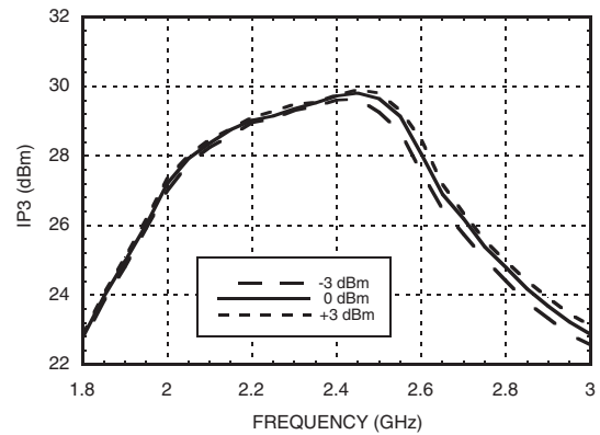
Upconverter Performance Input IP3 vs. LO Drive [1]
