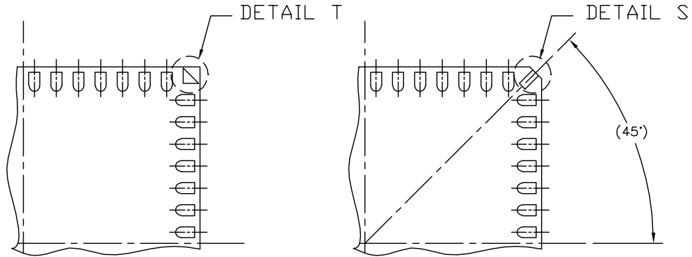
DETAIL M PREFERRED PIN 1 BACKSIDE IDENTIFIER
