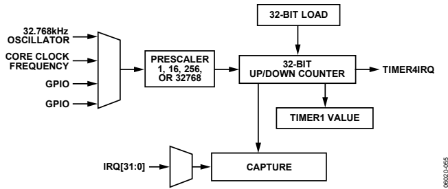
Figure 60. Timer4 Block Diagram
