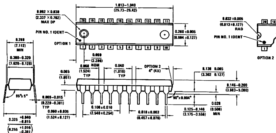
20-Lead Molded Dual-In-Line Package (N) Order Number DM74LS240N or DM74LS241N NS Package Number N20A
