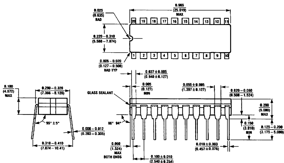
20-Lead Ceramic Dual-In-Line Package (J) Order Number DM54LS240J or DM54LS241J NS Package Number J20A
