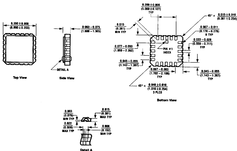
Ceramic Leadless Chip Carrier Package (E) Order Number DM54LS240E or DM54LS241E NS Package Number E20A
