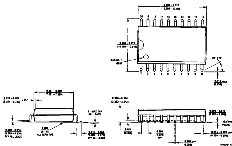
20-Lead Wide Small Outline Molded Package (M) Order Number DM74LS240WM or DM74LS241WM NS Package Number M20B
