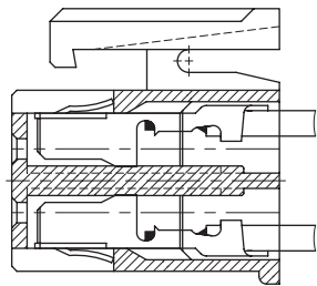
TERMINAL ASSEMBLY DRAWING
