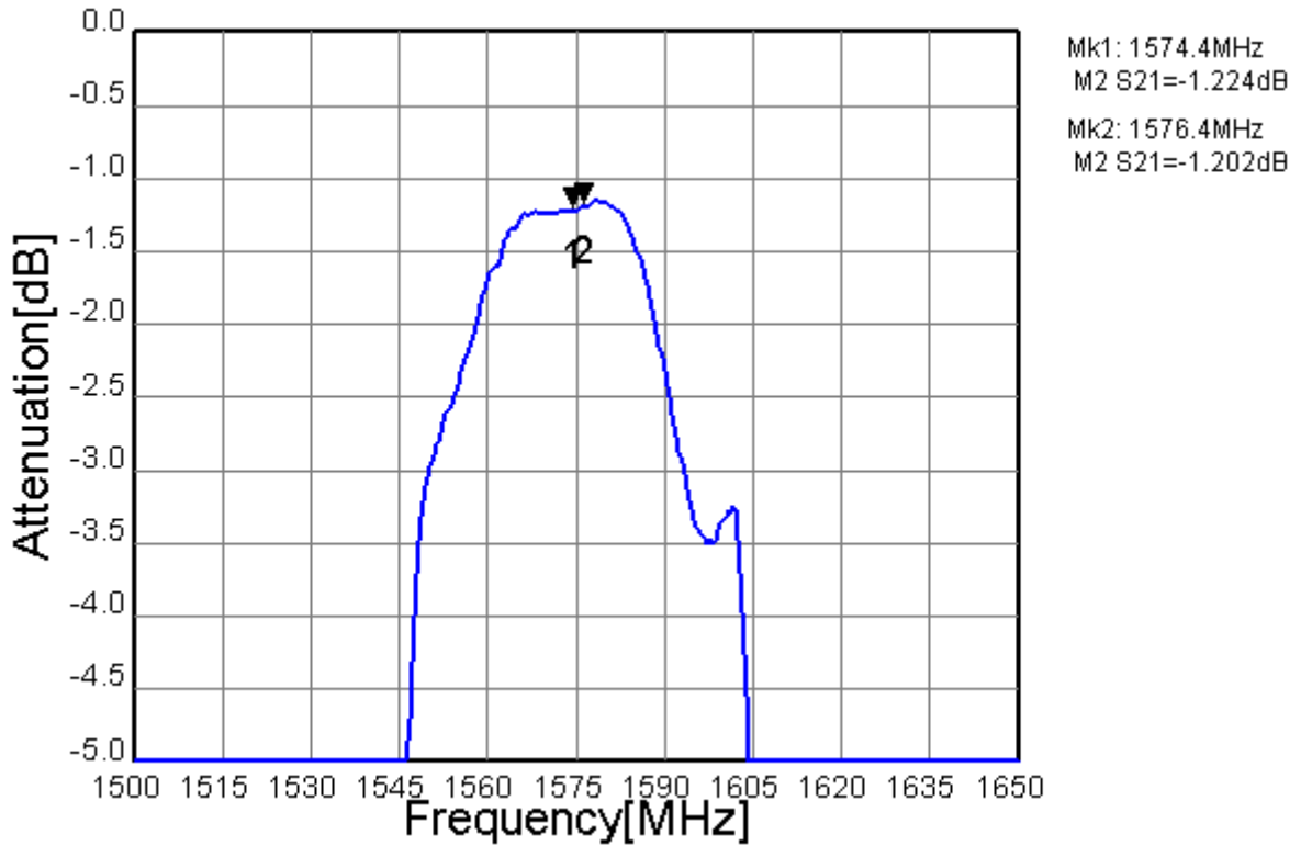
Fig.3 In-band Characteristic
