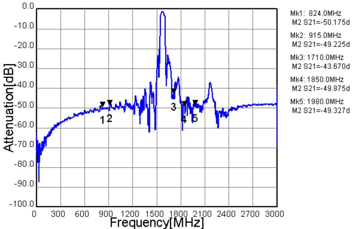
Fig.4 Wide-band Characteristic
