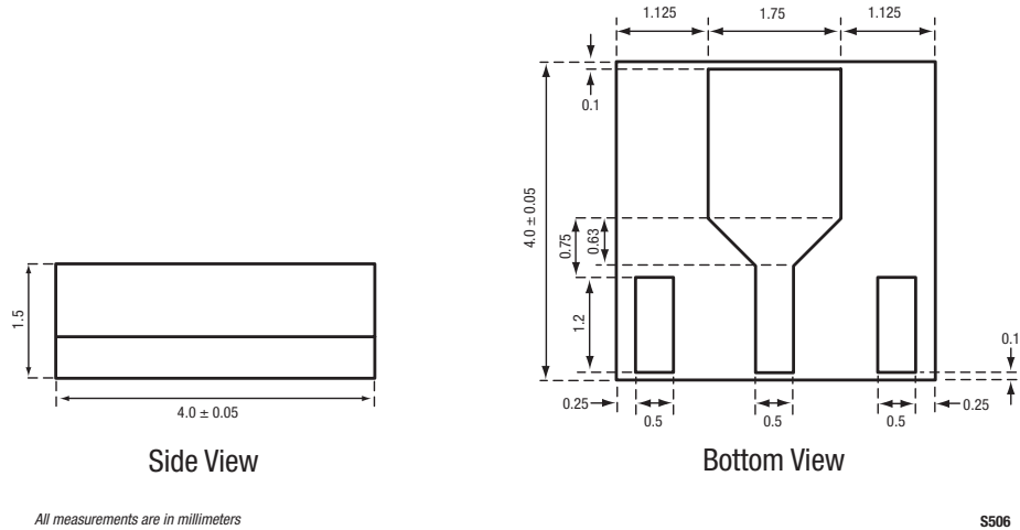
Figure 19. SKY65004-21 (3-Pin MCM) Package Dimensions
