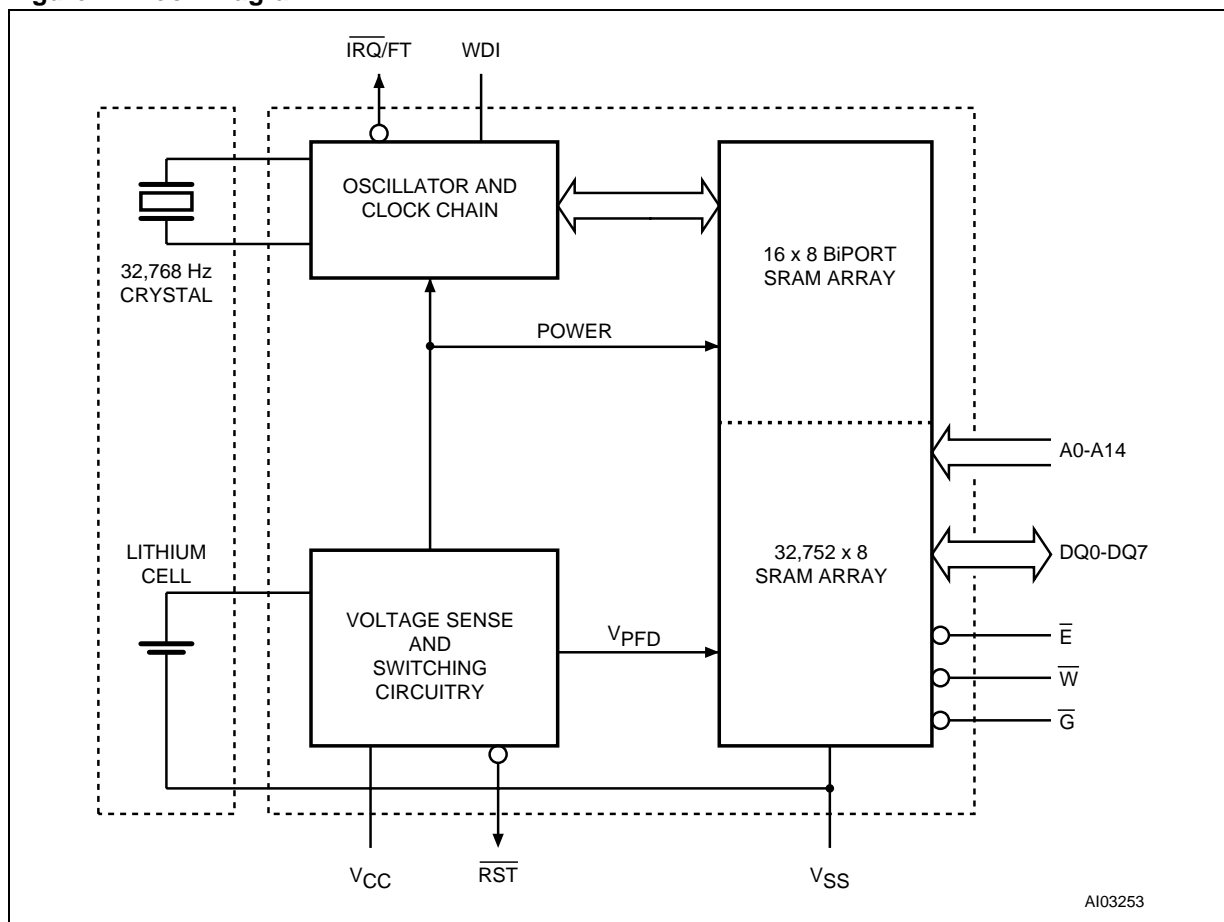
Figure 4. Block Diagram
