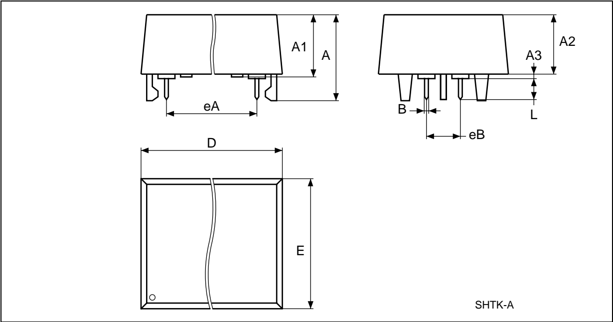
Figure 16. SH – 4-pin SNAPHAT Housing for 48mAh Battery & Crystal, Package Outline
