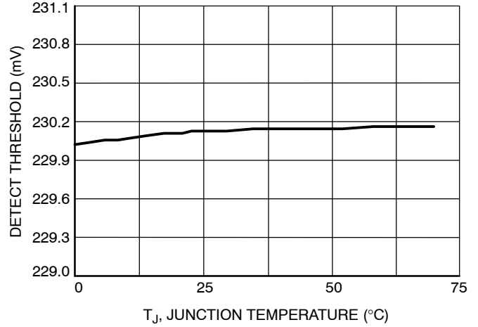
Figure 4. 2/3/4 Phase Detection Threshold vs. Temperature
