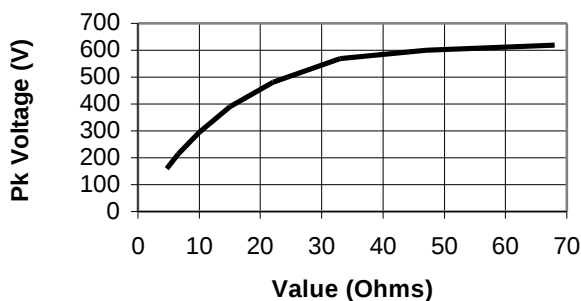
IEC61000-4-5 1.2/50ms Pulse
