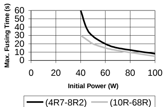
Fusing Characteristic (Constant Voltage)
