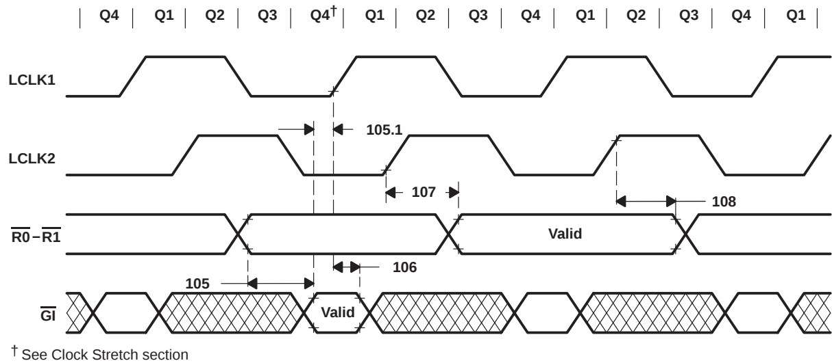
Figure 51. Multiprocessor Interface: \overline{GI} , \overline{ALTCH} , \overline{RAS} , \overline{R0} and \overline{R1}
