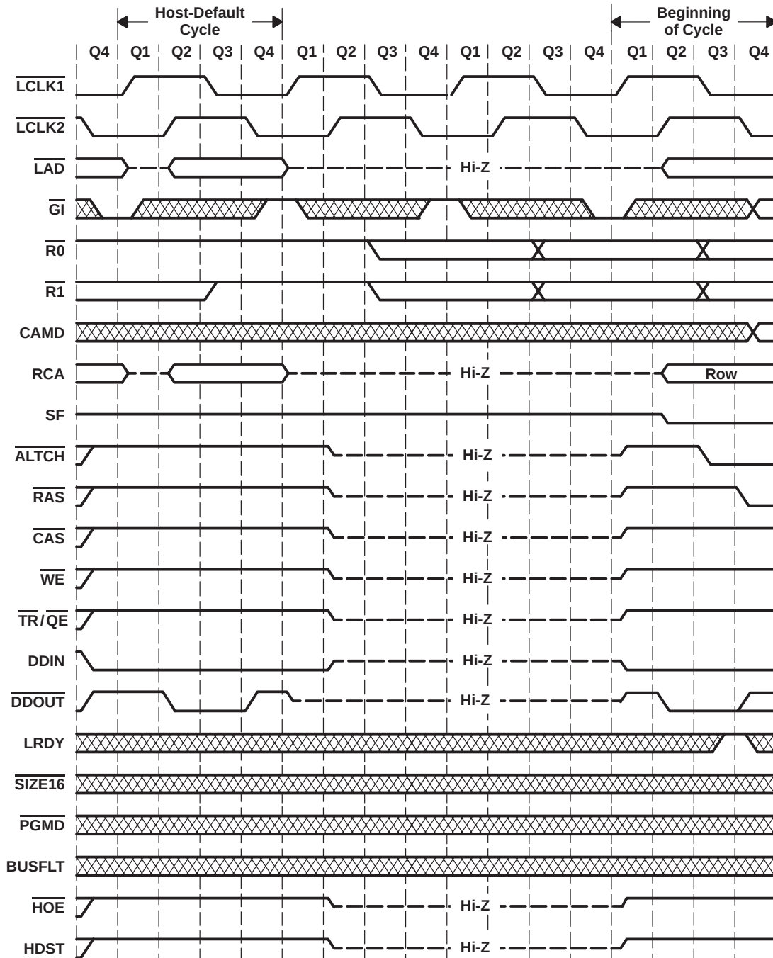
Figure 25. Multiprocessor-Interface Cycle (High-Impedance Signals)
