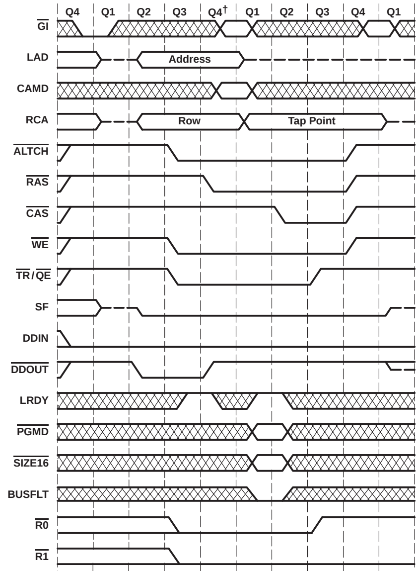
Figure 23. Serial-Data Register to Memory Cycle (VRAM-Write Transfer, Pseudo-Write Transfer)
