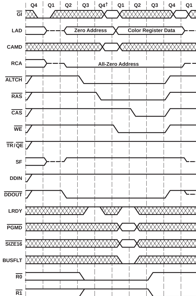
Figure 17. Load-Color-Latch Cycle
