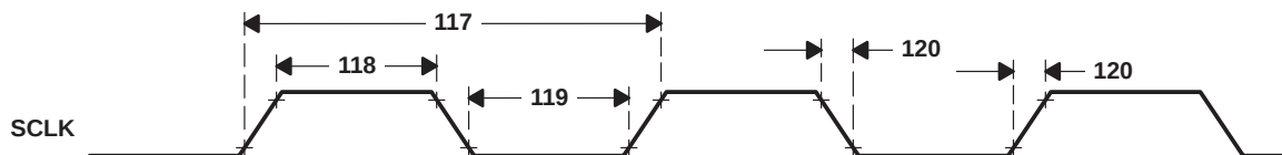
Figure 53. Video-Shift Clock: SCLK
