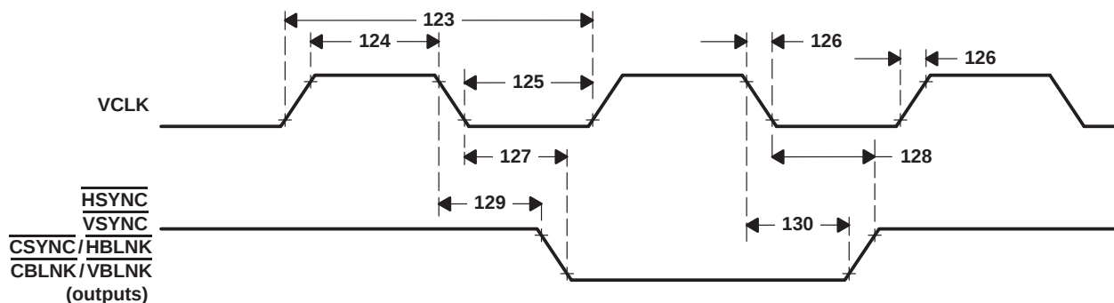
Figure 54. Video Interface: VCLK and Video Outputs
