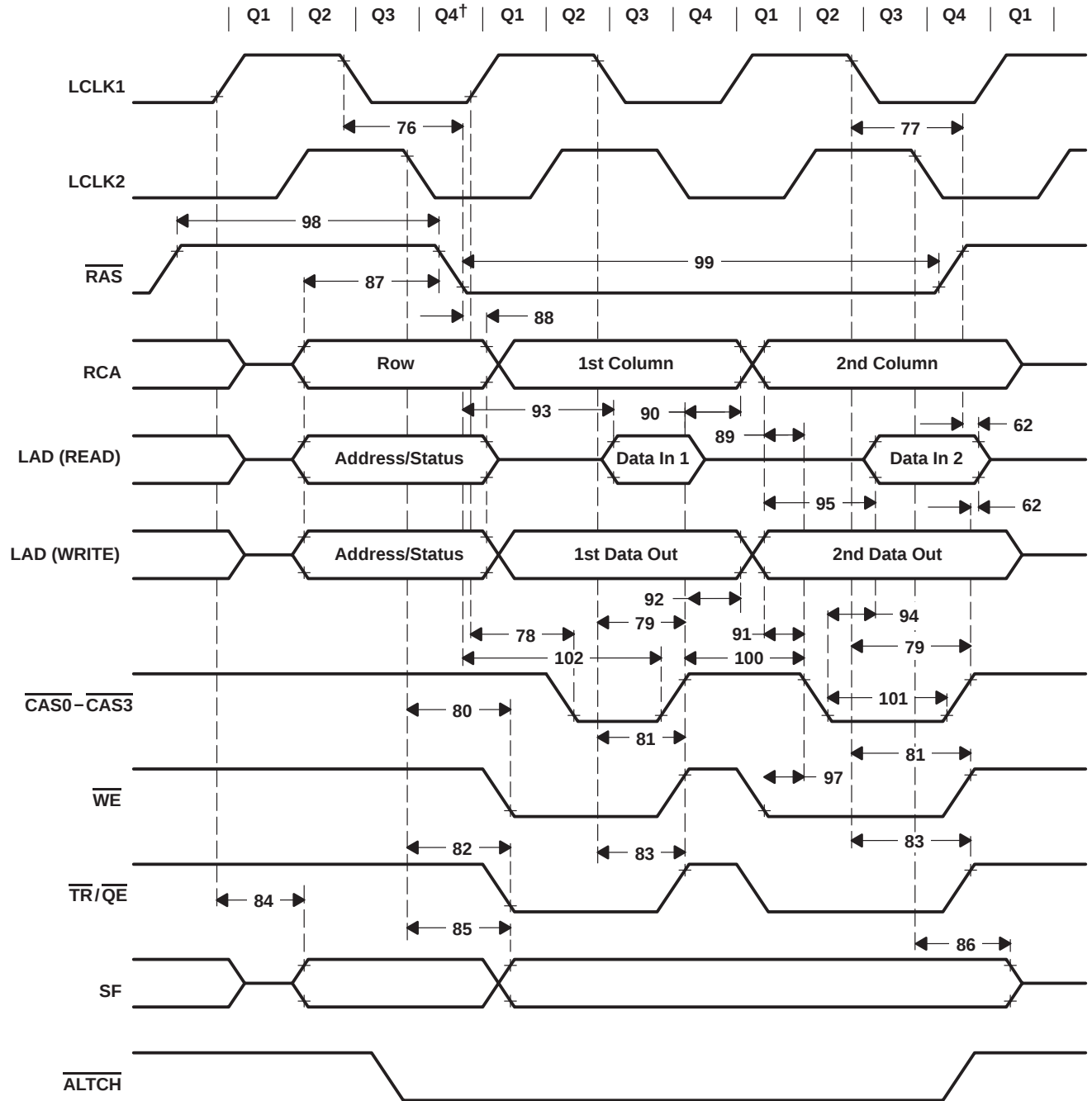
Figure 49. Local Bus: \overline{\text{RAS}} , \overline{\text{CAS0-CAS3}} , \overline{\text{WE}} , \overline{\text{TR/QE}} , and SF
