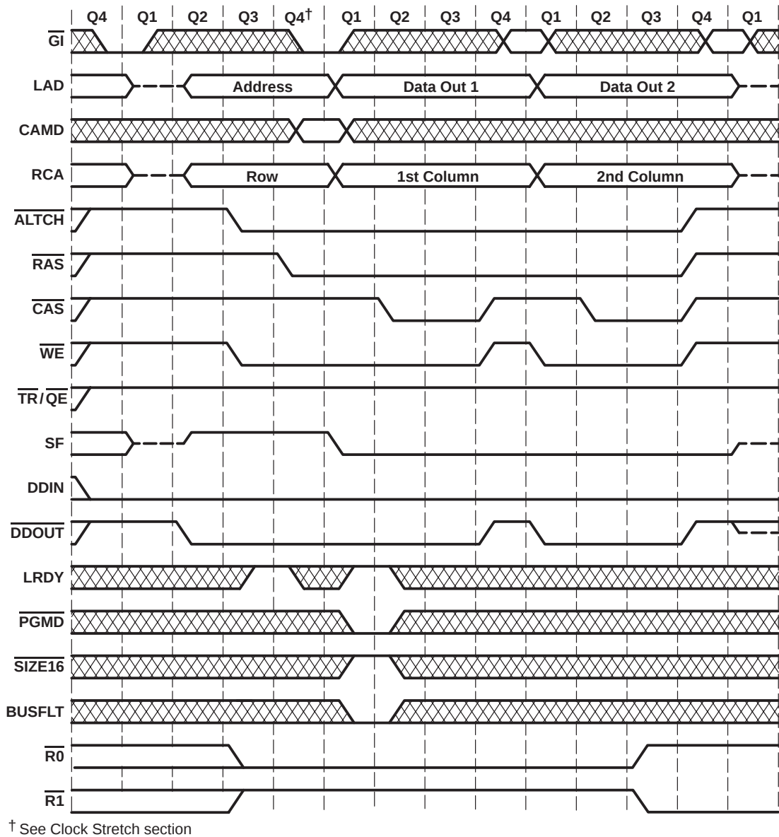
Figure 20. Write Cycle Using Mask
