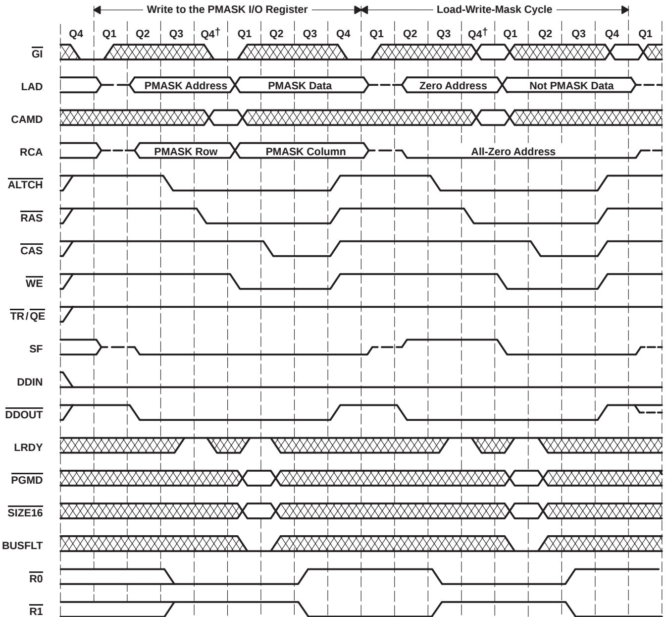
Figure 16. Load-Write-Mask Cycle
