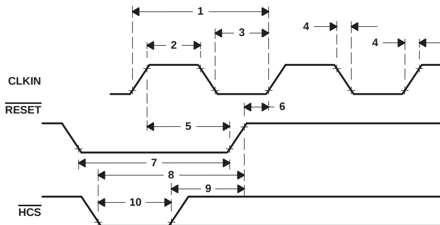
Figure 40. CLKIN and RESET
