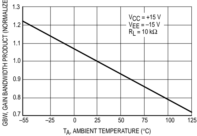
Figure 15. Normalized Gain Bandwidth Product versus Temperature
