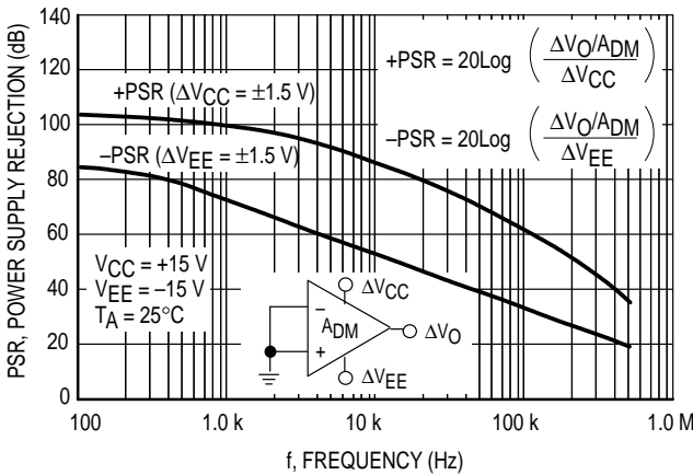
Figure 25. Power Supply Rejection versus Frequency
