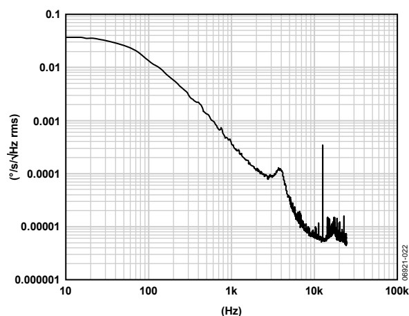
Figure 22. Noise Spectral Density with Additional 250 Hz Filter
