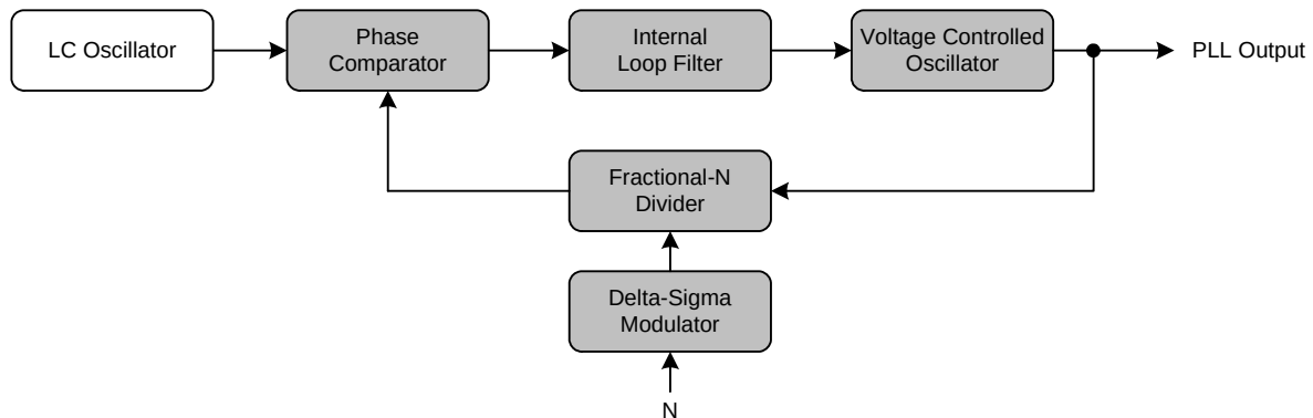
Figure 5. Delta-Sigma Fractional-N Frequency Synthesizer
