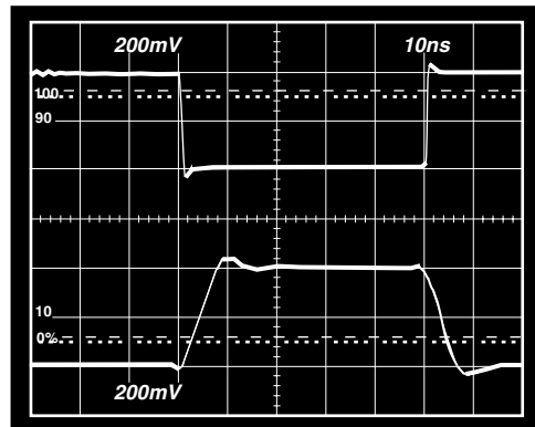
Figure 33. Inverter Small Signal Pulse Response \pm 5 V_S , C_F = 0 \text{ pF} , R_L = 150 \Omega
