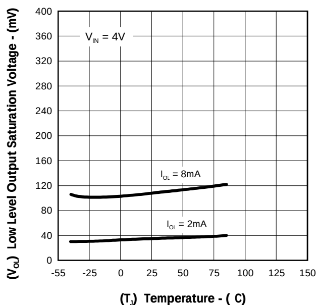
FIGURE 10. — LOW LEVEL OUTPUT SATURATION VOLTAGE vs. TEMPERATURE
