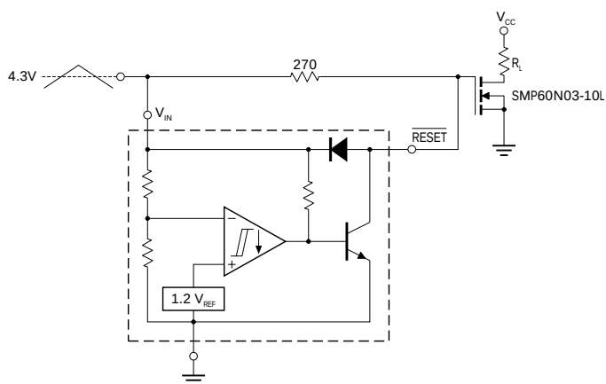
FIGURE 18. — MOSFET LOW VOLTAGE GATE DRIVE PROTECTION
