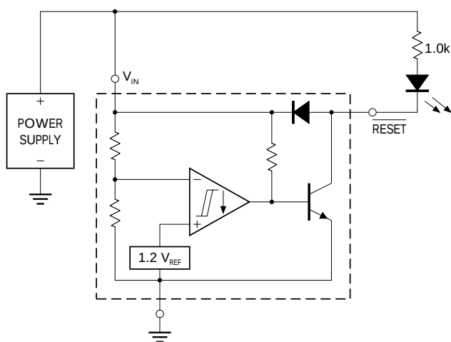
FIGURE 17. — VOLTAGE MONITOR
