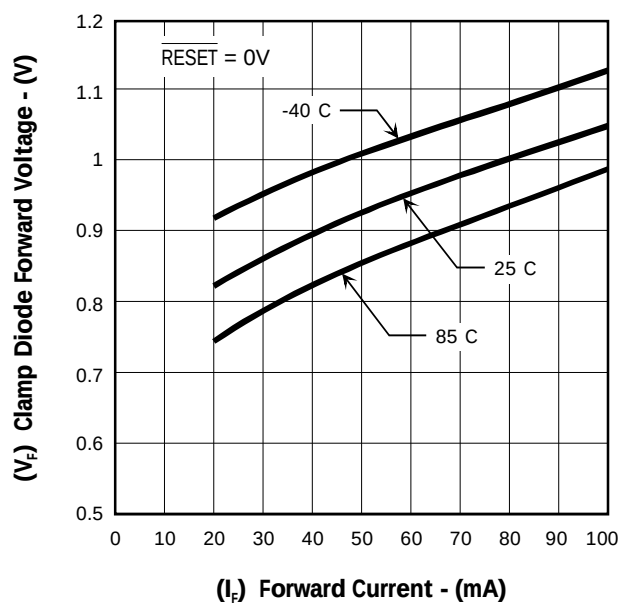
FIGURE 12. — CLAMP DIODE FORWARD VOLTAGE vs. FORWARD CURRENT
