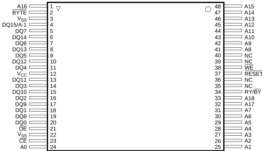
Reverse TSOP
