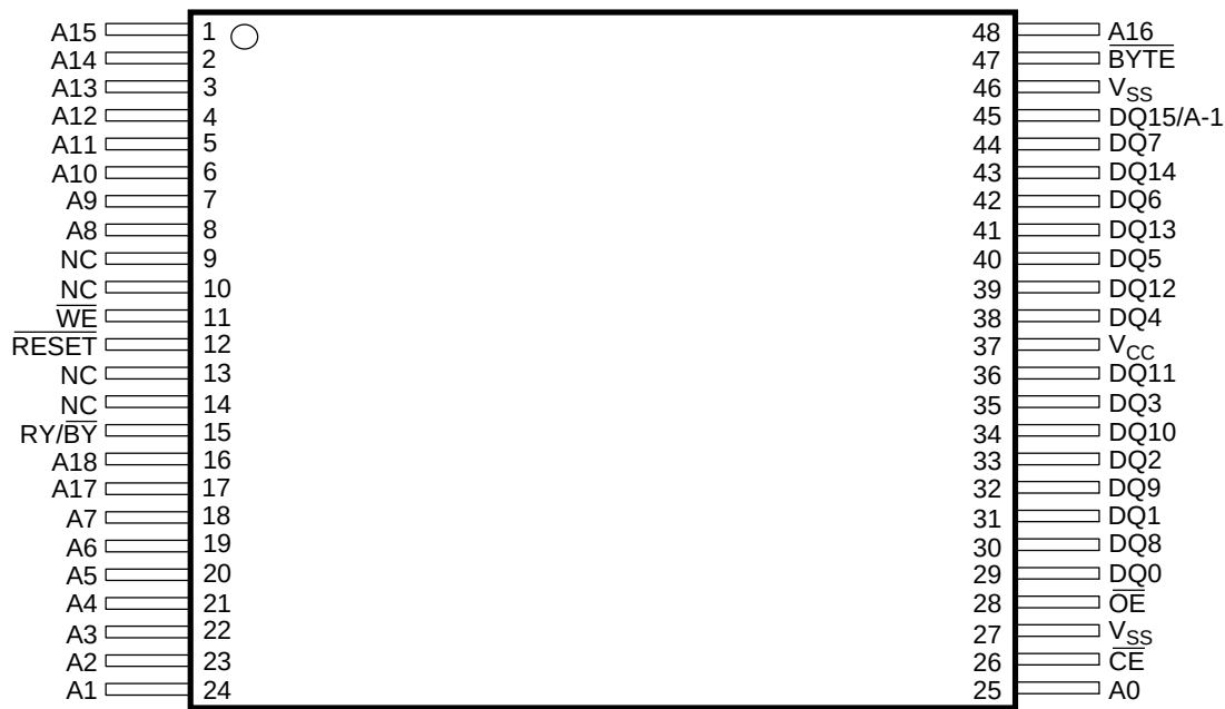
Standard TSOP
