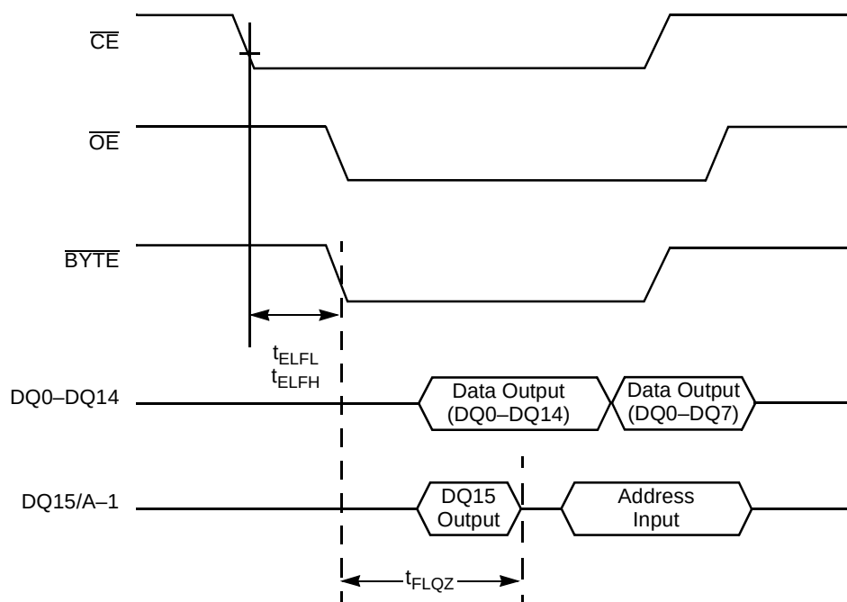
Figure 15. \overline{\text{BYTE}} Timing Diagram for Read Operation
