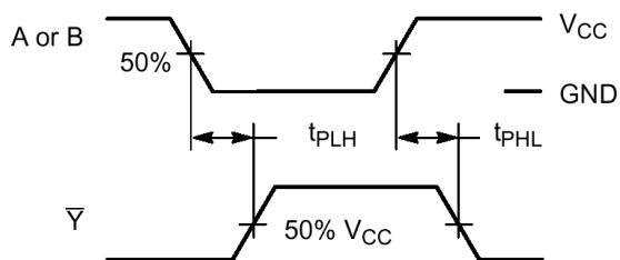
Figure 4. Switching Waveforms
