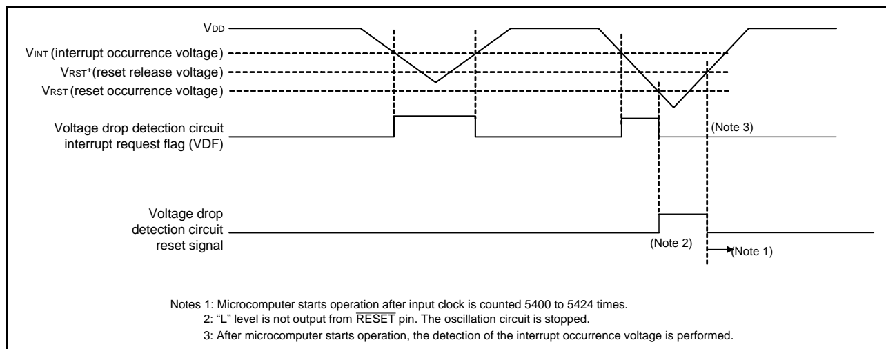
Fig 45. Voltage drop detection circuit operation waveform
