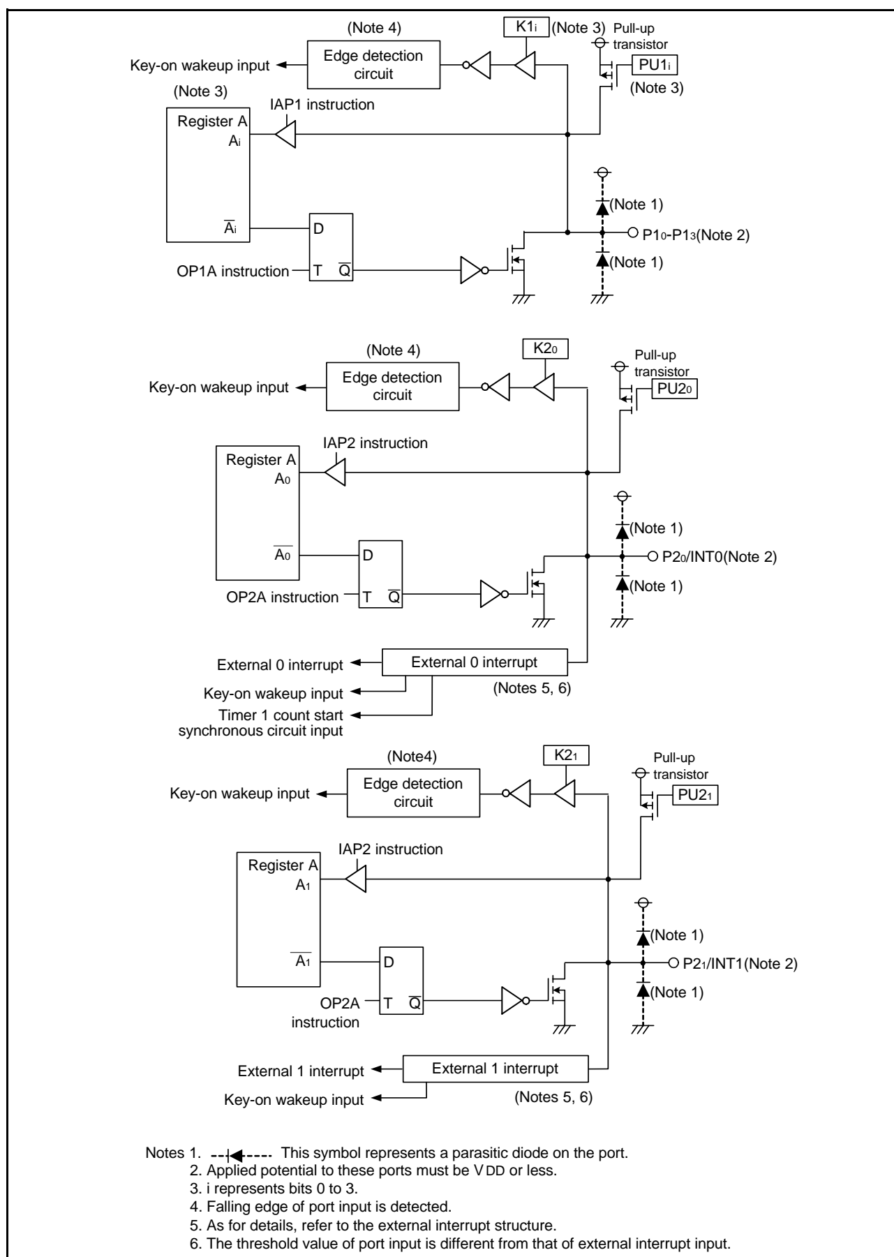
Fig 4. Port block diagram (2)
