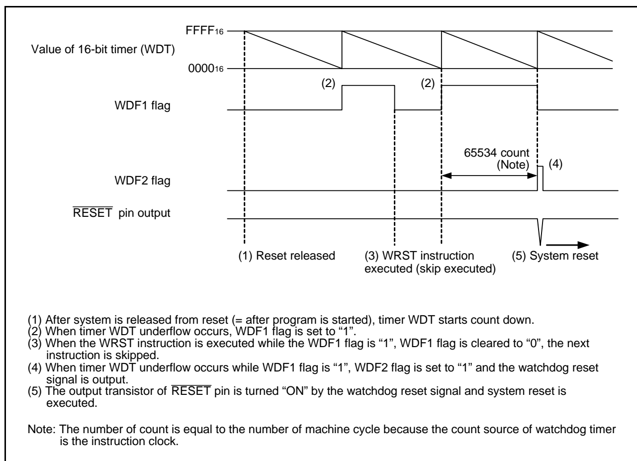
Fig 37. Watchdog timer function
