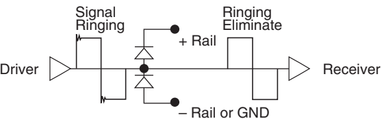
Signal Conditioning
