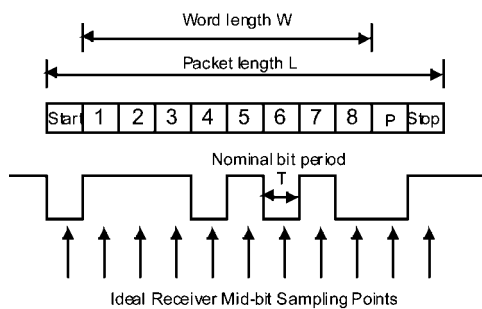
FIGURE 14. Nominal Mid-bit Sampling
