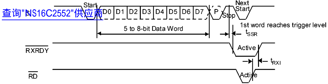
FIGURE 23. Receiver Timing FIFO Mode
