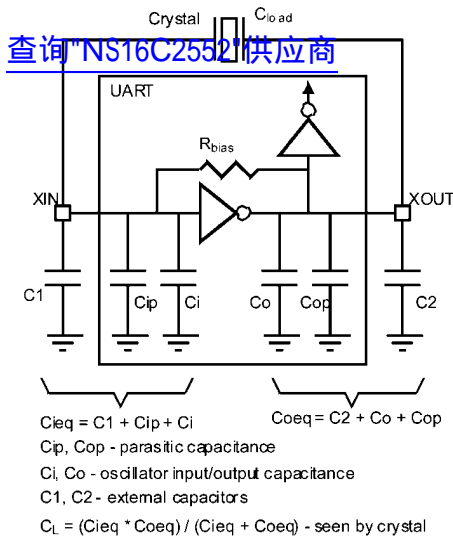
FIGURE 16. Crystal Oscillator Circuit
