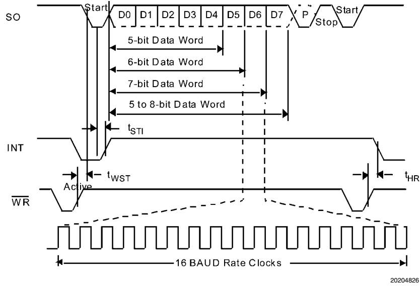
FIGURE 24. Transmitter Timing
