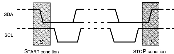
FIGURE 1. Start and Stop Conditions
