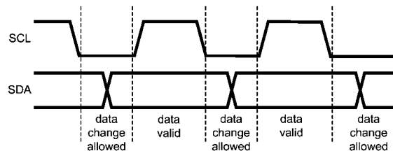
FIGURE 2. Data Validity Diagram
