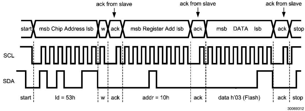
FIGURE 3. Write Cycle
