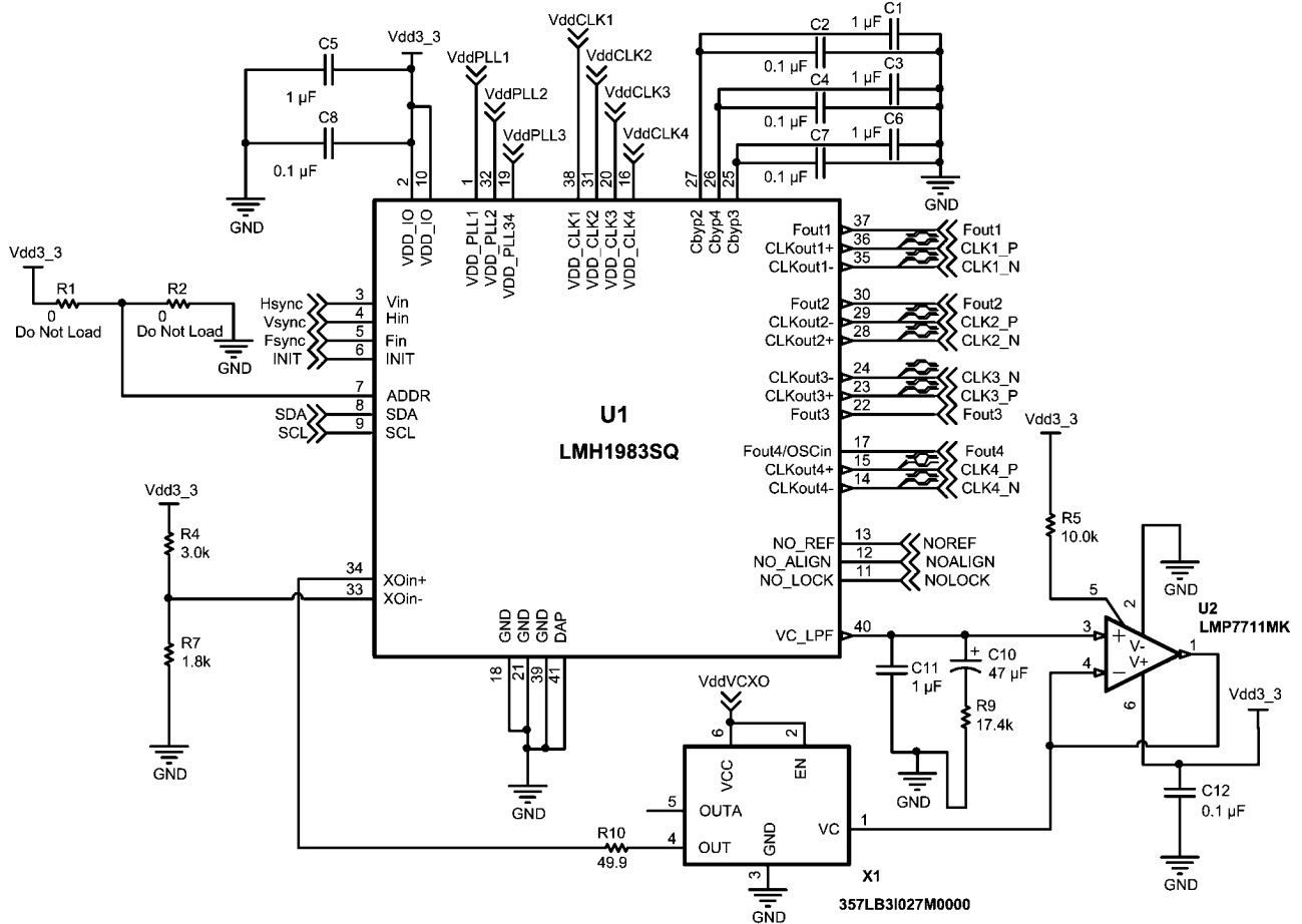
LMH1983 Typical Interface Circuit
