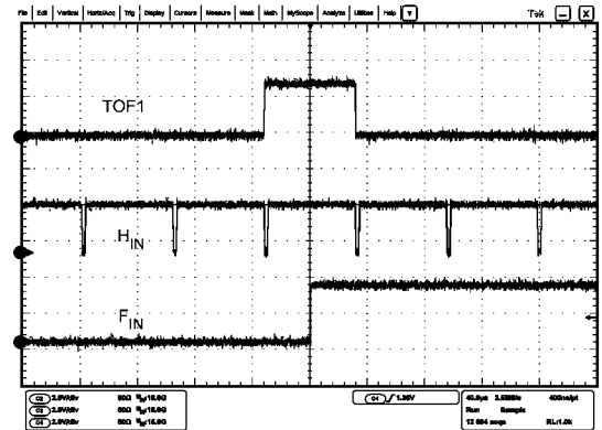
TOF1 Timing
