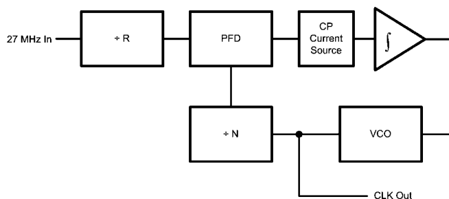
PLL2 / PLL3 Block Diagram
