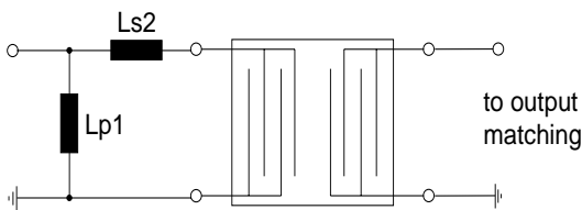
Fig. 3 shunt L – series L matching
