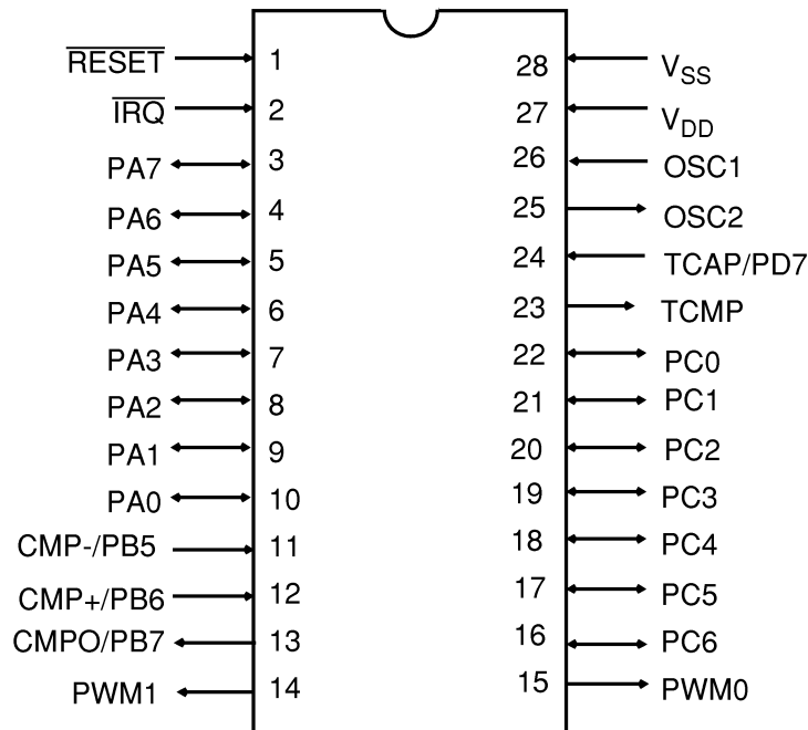
Figure 2-1: User Mode Pinout of the MC68HC05P5
