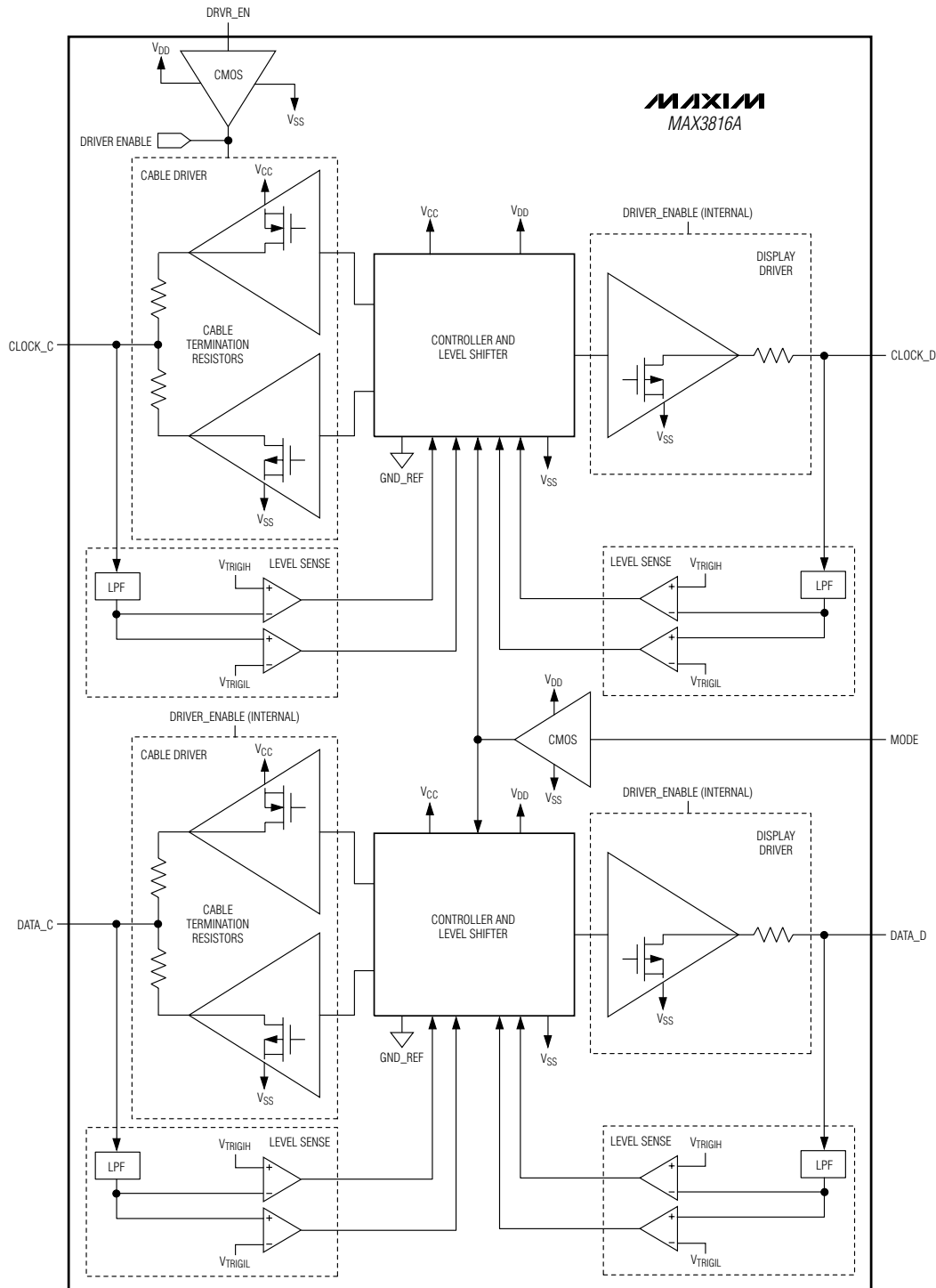
Figure 2. Functional Diagram
