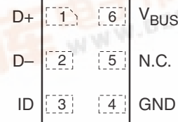
YFP PACKAGE (TOP VIEW)
