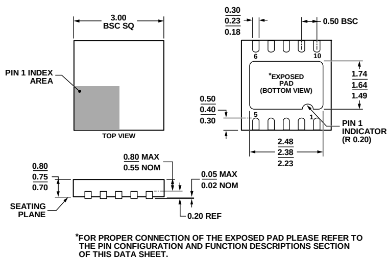
Figure 34. 10-Lead Lead Frame Chip Scale Package [LFCSP_WD] 3 mm × 3 mm Body, Very Very Thin, Dual Lead (CP-10-9) Dimensions shown in millimeters
