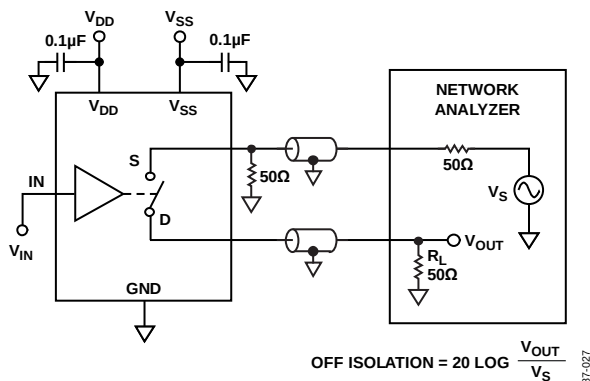
Figure 29. Off Isolation
