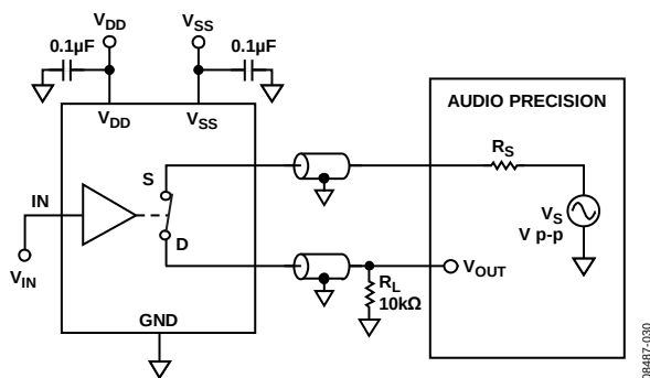
Figure 32. THD + N
