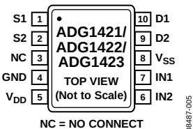
Figure 5. 10-Lead MSOP Pin Configuration
