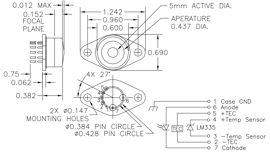
Mechanical Dimension in inches
