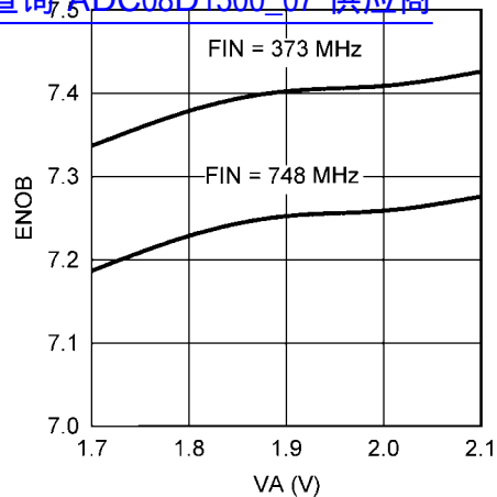
ENOB vs. SUPPLY VOLTAGE 查询"ADC08D1500_07"供应商
