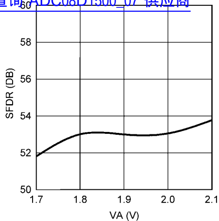
SFDR vs. SUPPLY VOLTAGE 查询"ADC08D1500_07"供应商
