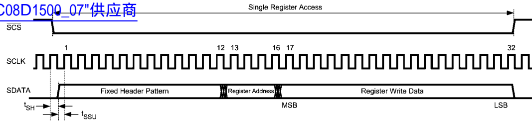
FIGURE 5. Serial Interface Timing
