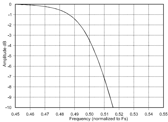
Figure 21. Transition Band
