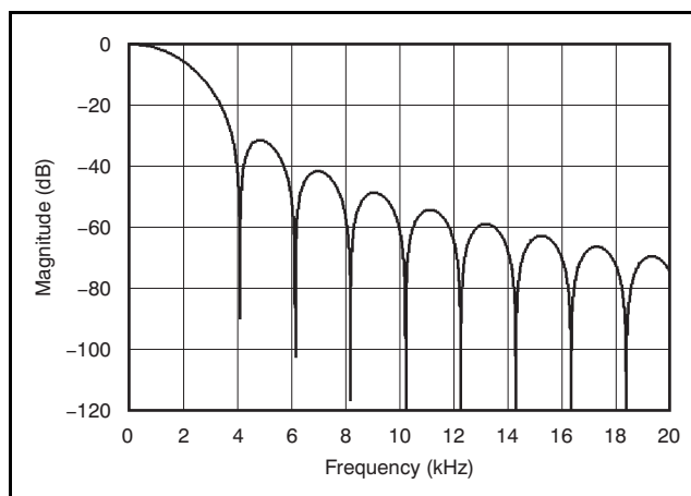
Figure 61. Filter Profile with Data Rate = 2kSPS
