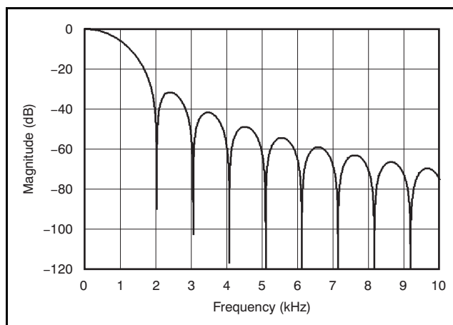
Figure 60. Filter Profile with Data Rate = 1kSPS
