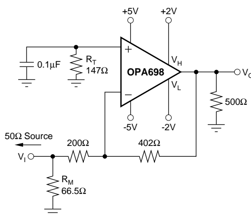
Figure 49. Inverting G = -2 Specifications and Test Circuit
