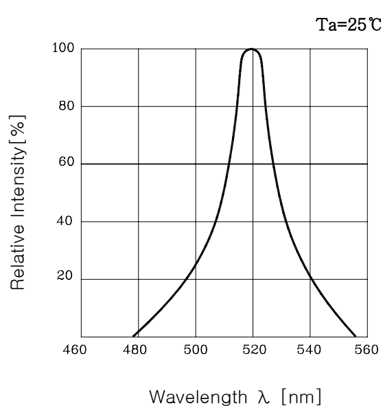
Fig. 4 Spectrum Distribution
