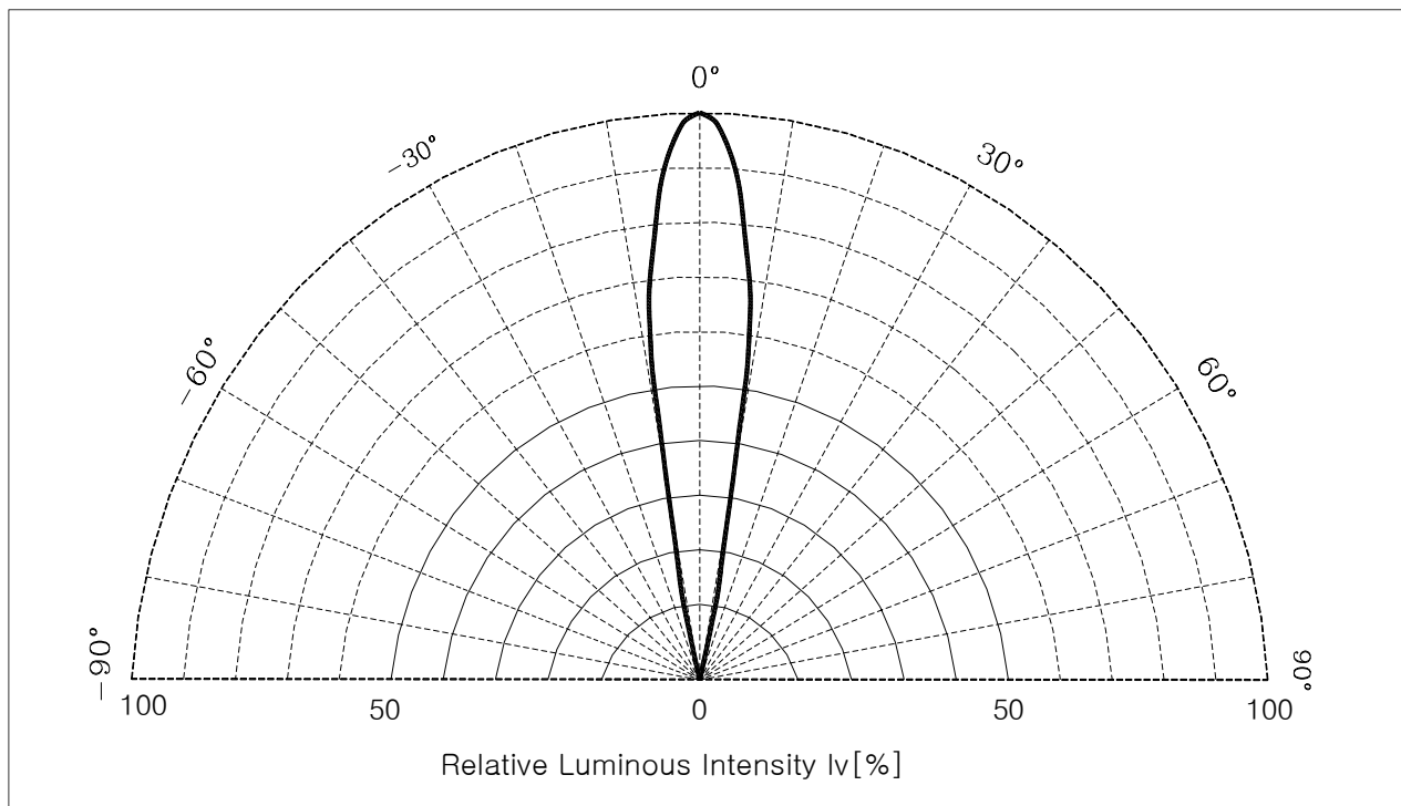
Fig. 5 Radiation Characteristics
