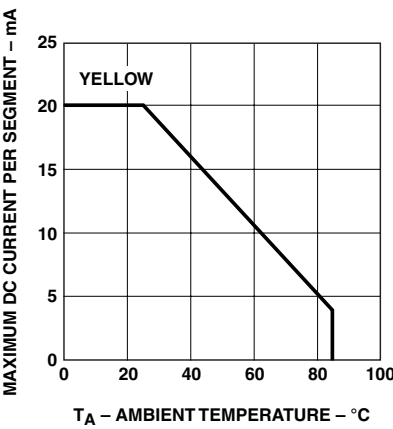
Figure 13. Maximum allowable average or DC current vs. ambient temperature.
