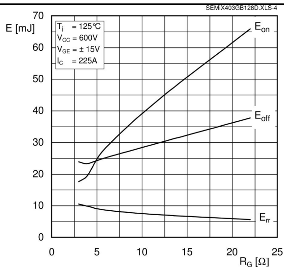
Fig. 4 Typ. turn-on /off energy = f(R_G)
