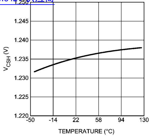
V CSH vs. Junction Temperature 查询"LM3424"供应商
