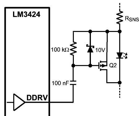
FIGURE 18. Buck Level-Shifted PWM Circuit
