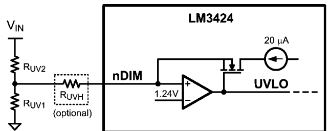
FIGURE 15. UVLO Circuit
