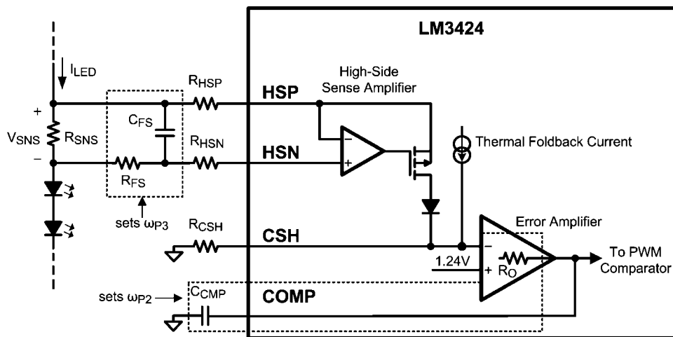
FIGURE 10. Compensation Circuitry
