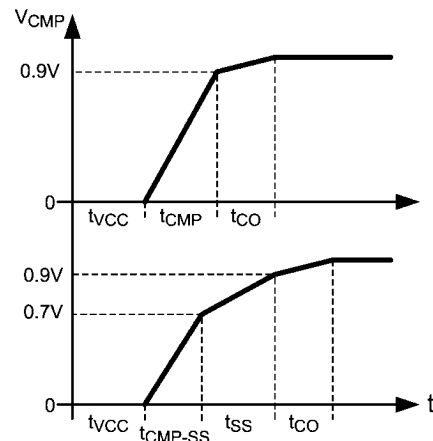
FIGURE 12. Start-up Waveforms
