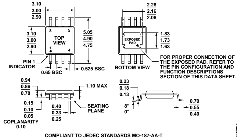
Figure 45. 8-Lead Mini Small Outline Package with Exposed Pad [MINI_SO_EP] (RH-8-1) Dimensions shown in millimeters
