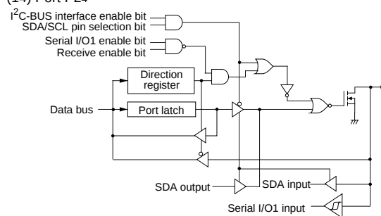
(14) Port P24
