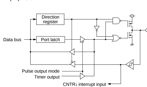
(18) Port P40
