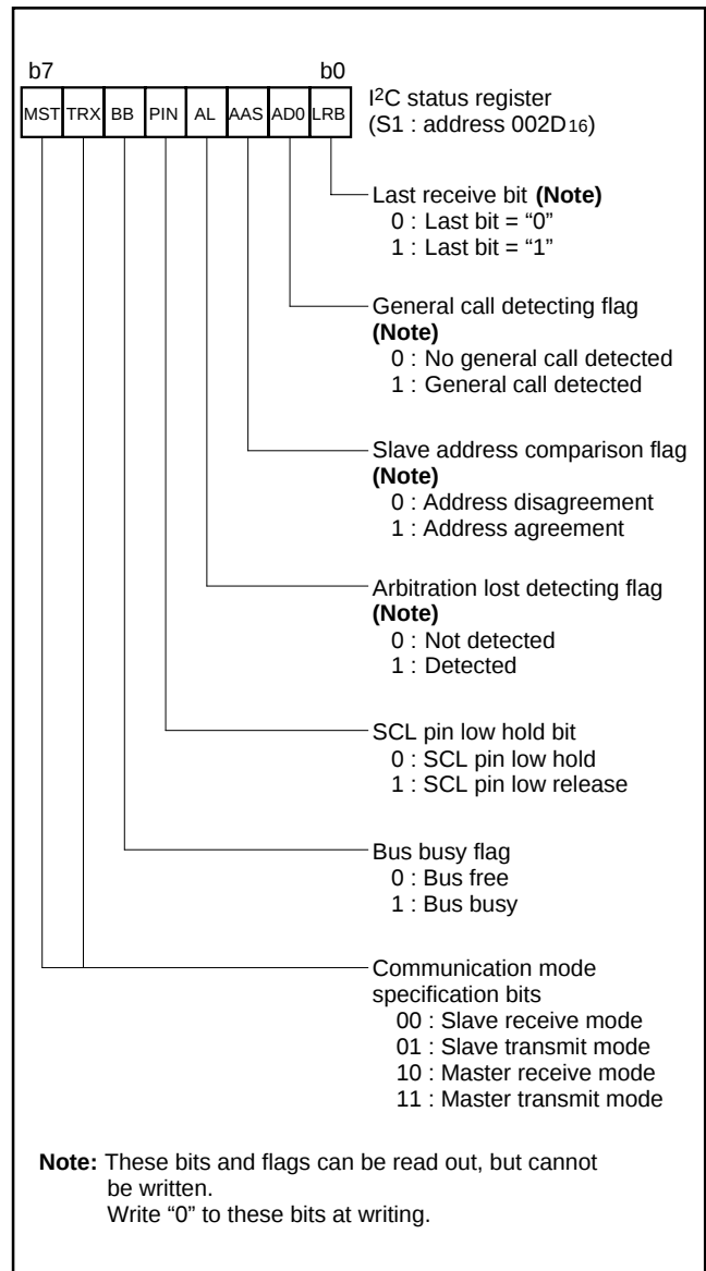
Fig. 31 Structure of I²C status register
