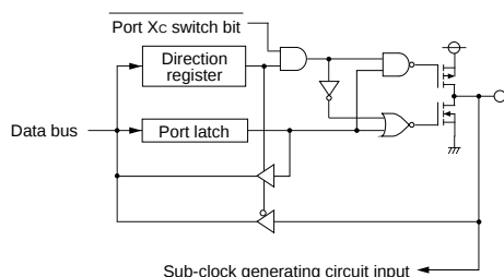
(11) Port P21
