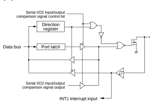
(20) Port P43
