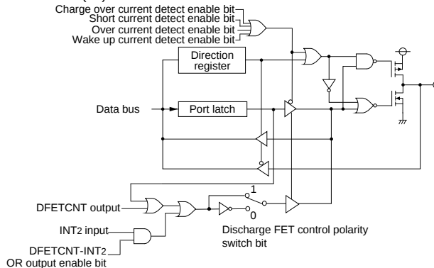
(22) Port P45
