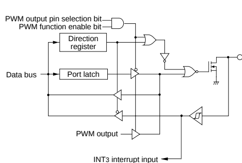
(21) Port P44
