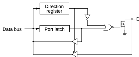
(9) Port P1
