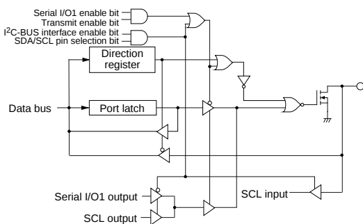
(15) Port P25
