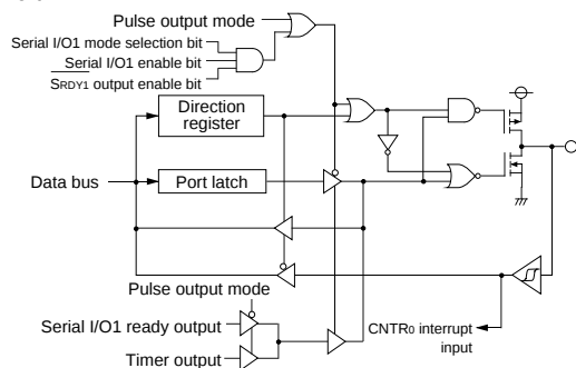
(17) Port P27
