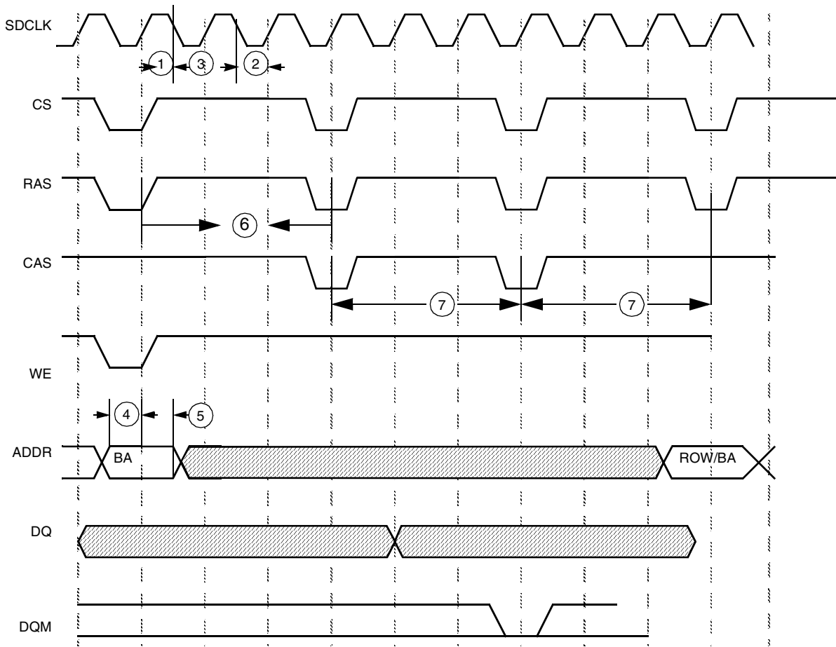
Figure 32. SDRAM Refresh Timing Diagram
