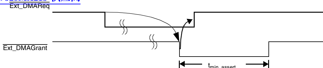
Figure 4. Assertion of DMA External Grant Signal
