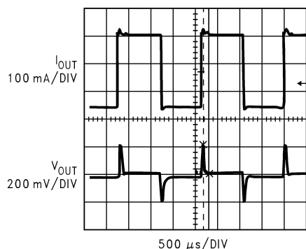
FIGURE 5. 130mA to 400mA Transient Response of the circuit in Figure 9 with C_{FF} = 1nF
