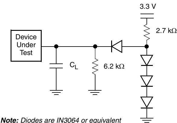
Figure 12. Test Setup
