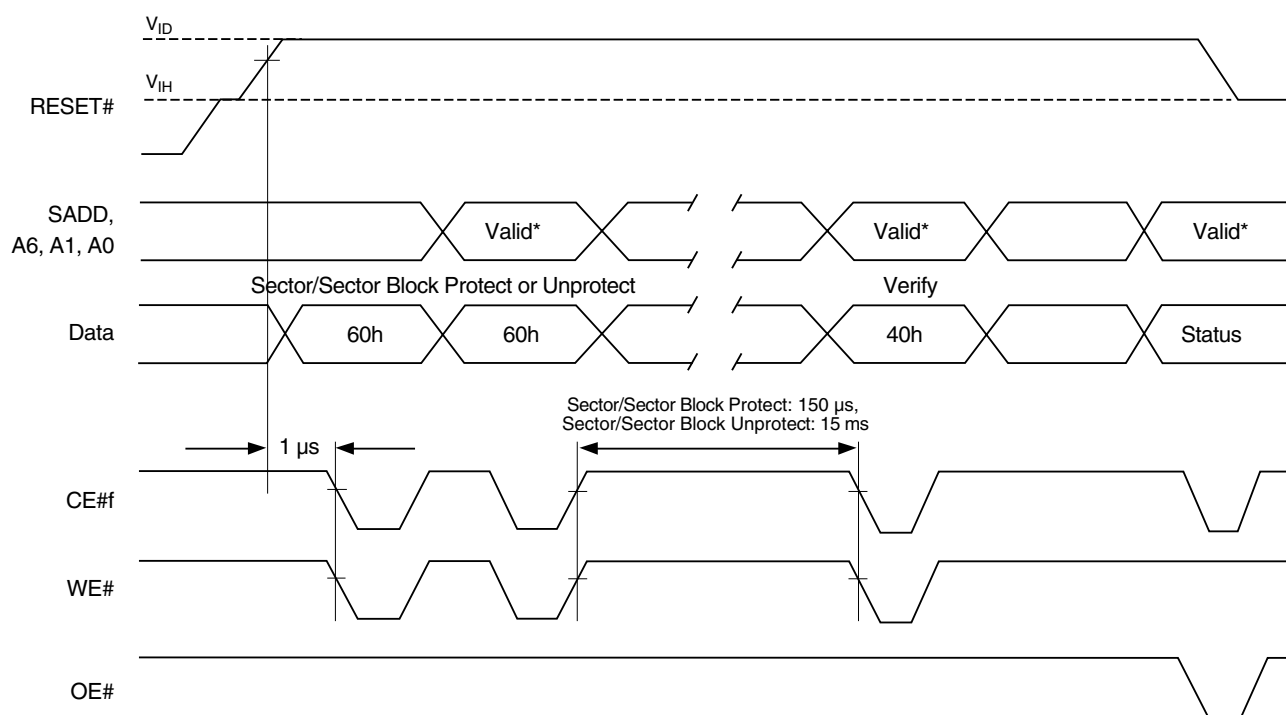
Figure 25. Sector/Sector Block Protect and Unprotect Timing Diagram
