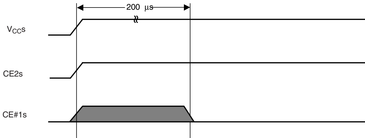
Figure 27. Power Up
