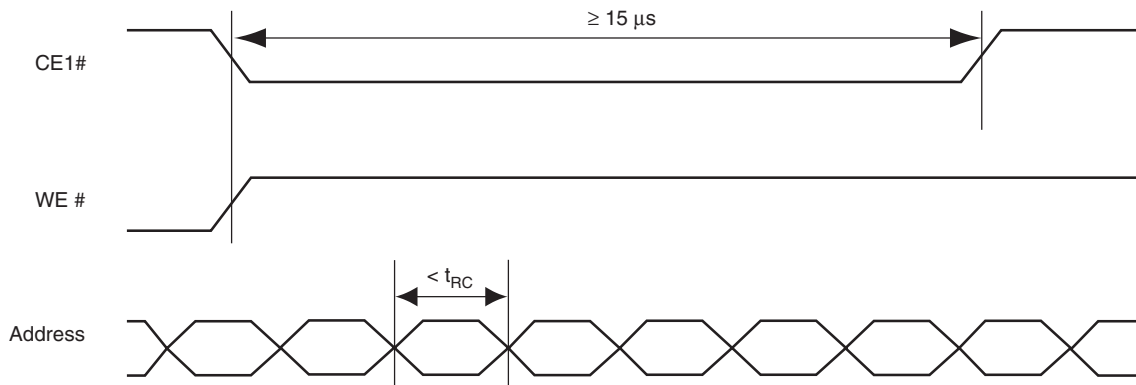
Figure 35. Abnormal Timing
