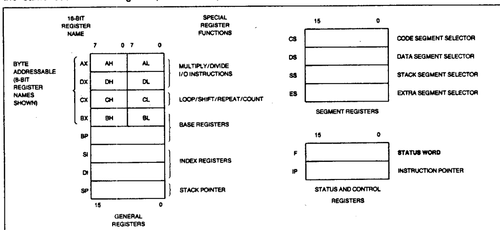
Figure 3. Register Set
