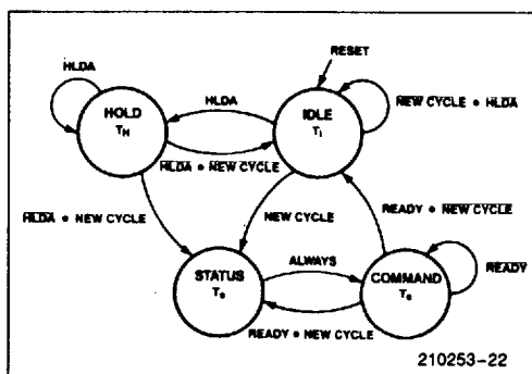
Figure 22. 80286 Bus States
