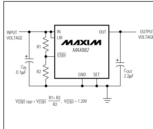
Figure 3. Setting an Undervoltage Lockout Threshold Using STBY
