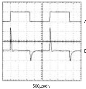
LINE-TRANSIENT RESPONSE
