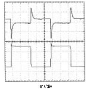
LOAD-TRANSIENT RESPONSE
