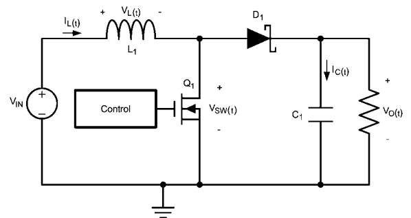
FIGURE 2. Simplified Schematic
