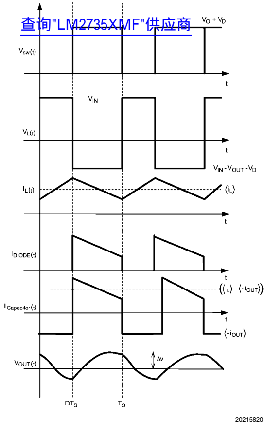
FIGURE 3. Typical Waveforms
