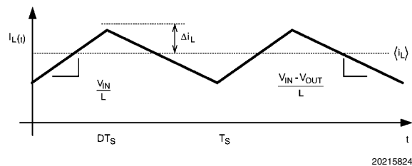
FIGURE 4. Inductor Current
