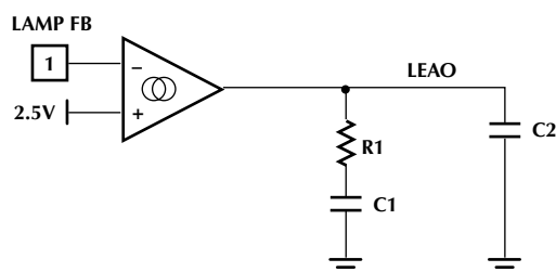
Figure 4. Compensation Network
